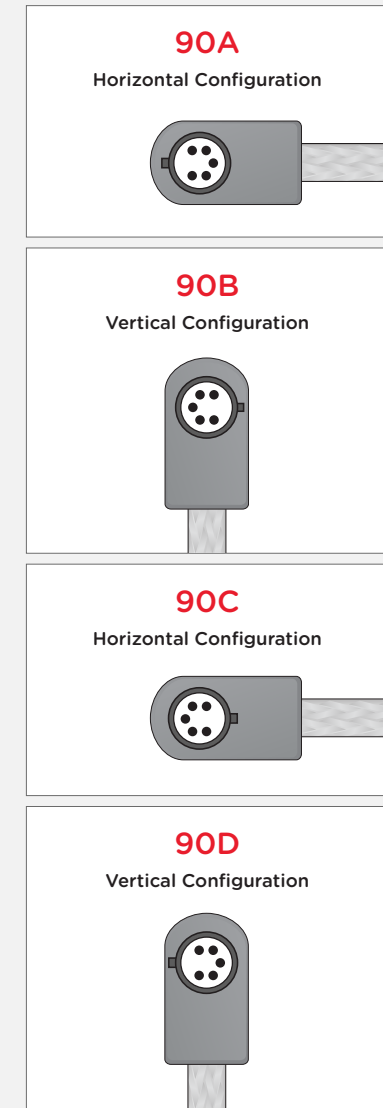
Pin Orientation of 90° (Right Angle) DIN Connector
